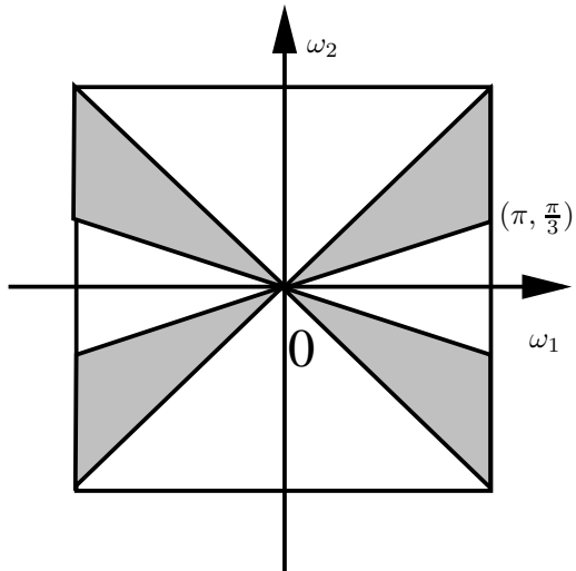
Fig. 3. Specifications of the fan filter in Example 2.
