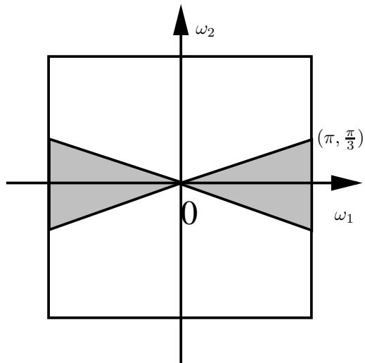
Fig. 1. Specifications of the fan filter in Example 1.
