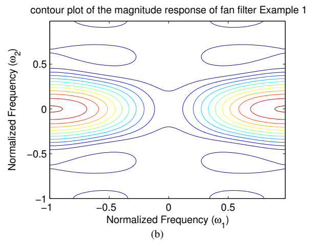
Fig. 2. (a) The magnitude response of the designed filter in Example 1. (b) The corresponding contour plot.
