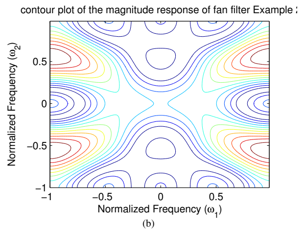
Fig. 4. (a) The magnitude response of the designed filter in Example 2. (b) The corresponding contour plot.
